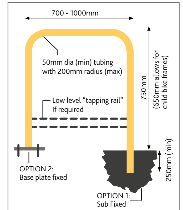
Diagram 3: Sheffield stand (London) Cycling Design Standards, TfL 2014)
